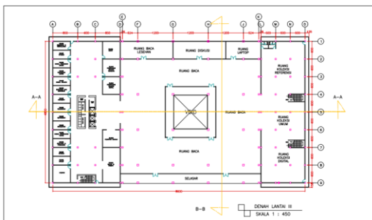
Gambar 5. Denah Lantai 3
