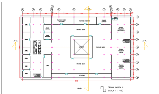
Gambar 4. Denah Lantai 2
